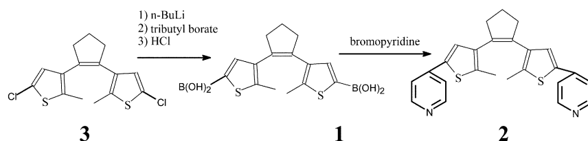
Scheme 2 Synthetic route of the compound 2 in the study.
